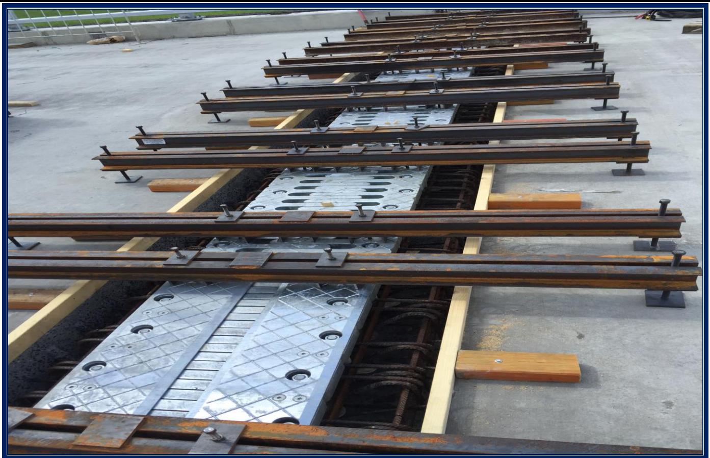
EJC and brackets before concreting
